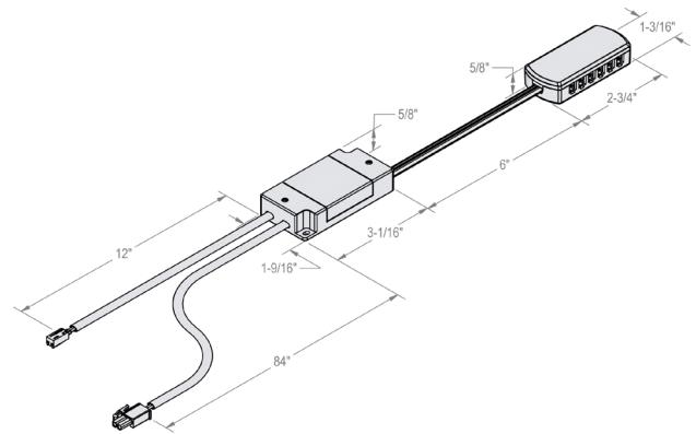
Part No. PS24V/DIM/EURO
